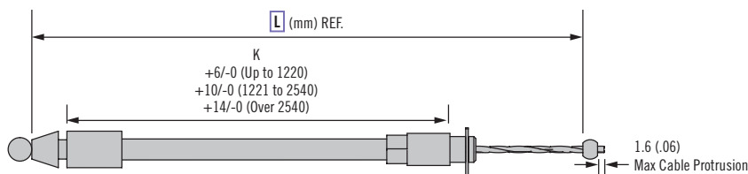
Type 6 - Jacketed Cable with Snub End Coupling and Threaded Retainers (P/N AC-CAC1-6- L -048 as shown)
