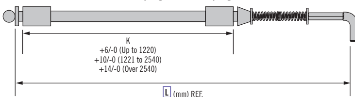
Type 7 - Jacketed Cable with Snub End Coupling and End Coupling Retainers (P/N AC-CAB1-7- L -048 as shown)
