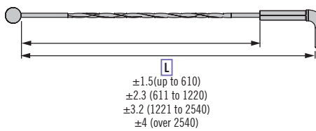
Type 3 - Jacketed Cable with End Coupling Retainers (Shown with Spring Option) (P/N AC-CBB1-3- L -048 as shown)
