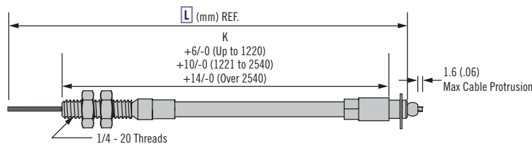
Type 5 - Jacketed Cable with Snap Ring and End Coupling Retainers (P/N AC-CAH0-5- L -048 as shown)
