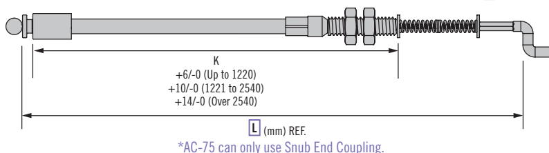
Type 7 - Jacketed Cable with Snub End Coupling and End Coupling Retainers (P/N AC-CAB1-7- L -048 as shown)
