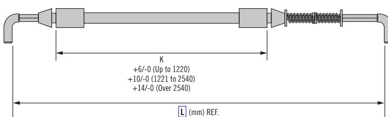
Type 3 - Jacketed Cable with End Coupling Retainers (Shown with Spring Option) (P/N AC-CBB1-3- L -048 as shown)
